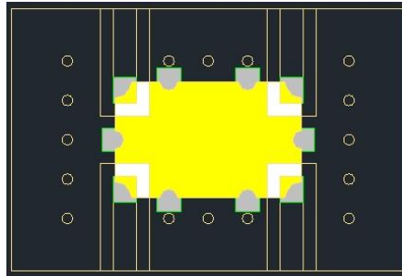
Figure 11. Placing the CMX03A03 on the 9 Points of the PCB Surface
