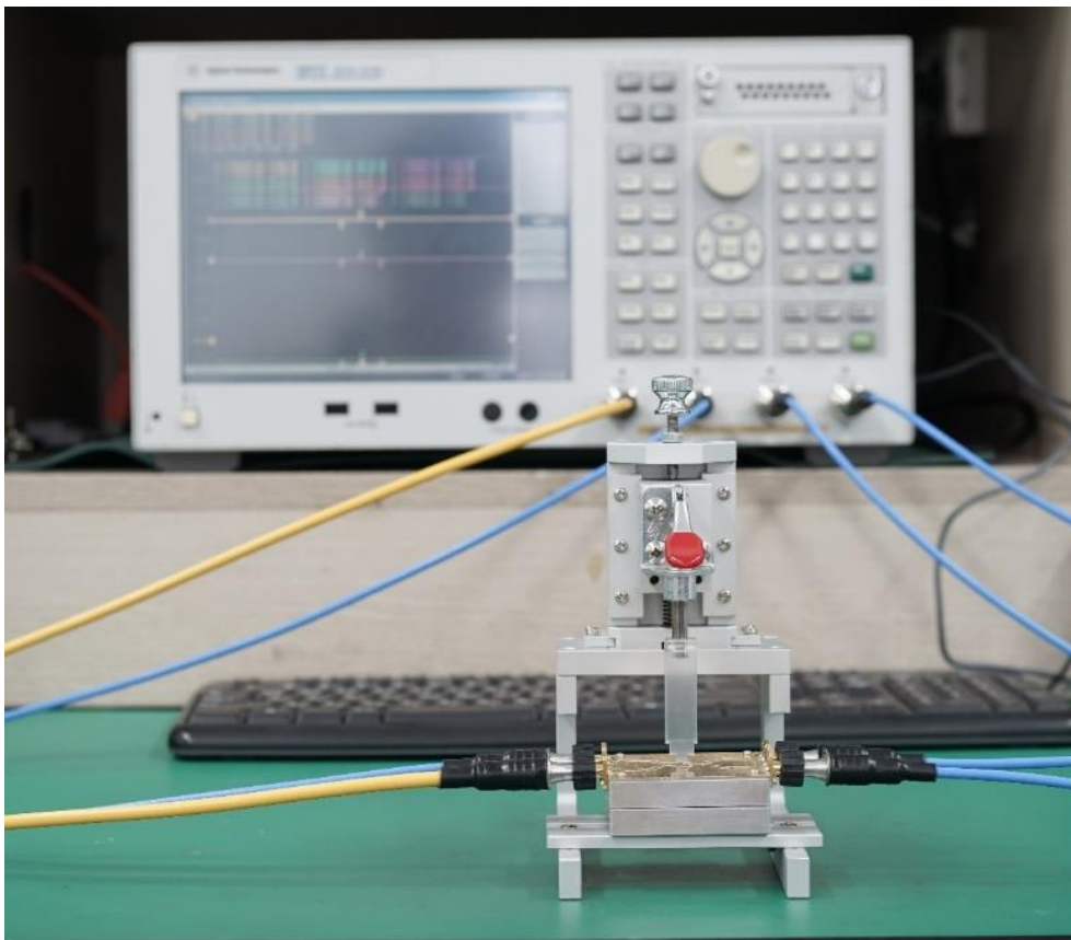
Figure 5. Test Setting to Measure the CMX03A03 S-parameters
