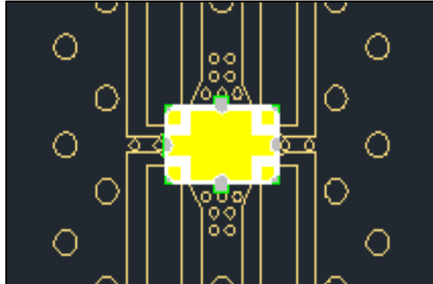
Figure 11. Placing the CMX07E03 on the 9 Points of the PCB Surface
