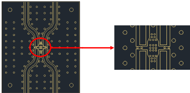
Figure 9. Cleaning the PCB Surface Where the CMX07E03 is Soldered
