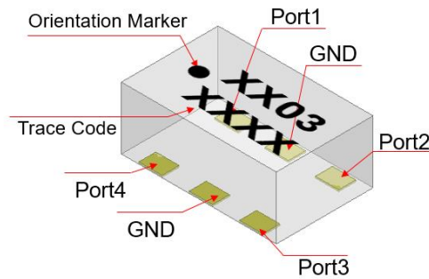
Figure 1. Top View
