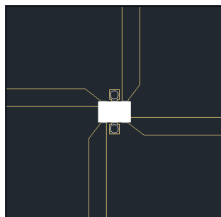
Figure 11. Placing the CMX15P03 on the 6 Points of the PCB Surface
