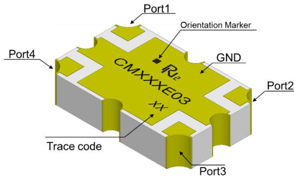
Figure 1. CMX19E03 (Top View)
