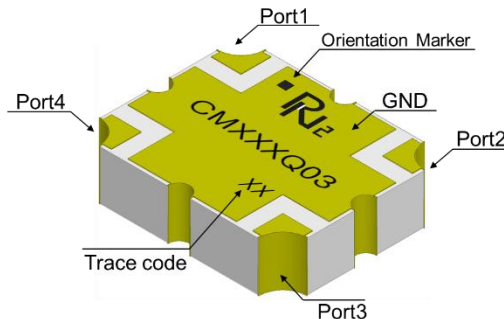
Figure 1. CMX20Q03 (Top View)
