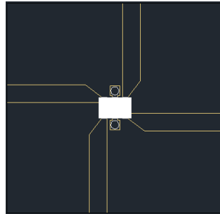
Figure 11. Placing the CMX35P03 on the 6Points of the PCB Surface
