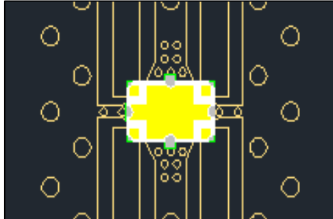
Figure 11. Placing the CMX45E03 on the 9 Points of the PCB Surface
