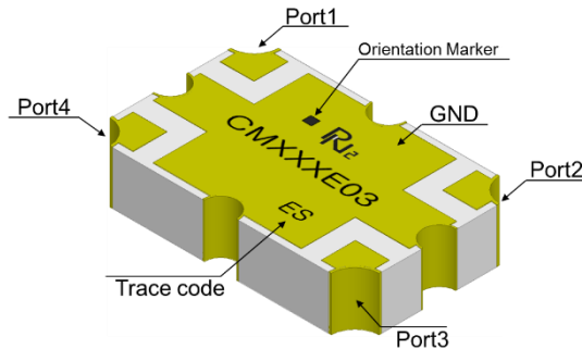
Figure 1. CMX45E03 (Top View)
