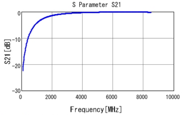
GRM1555C1H1R2WA01 S21 DCOV, 25degC
