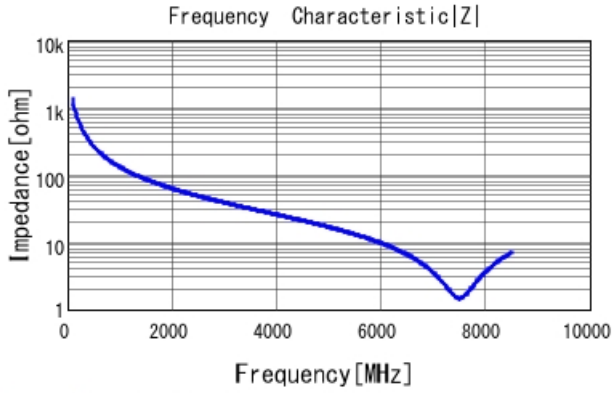
GRM1555C1H1R2WA01 |Z| DCOV, 25degC
