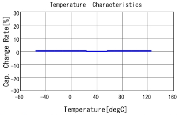
GRM1555C1H1R2WA01 C-Temp. capchange, DCOV, AC1Vrms
