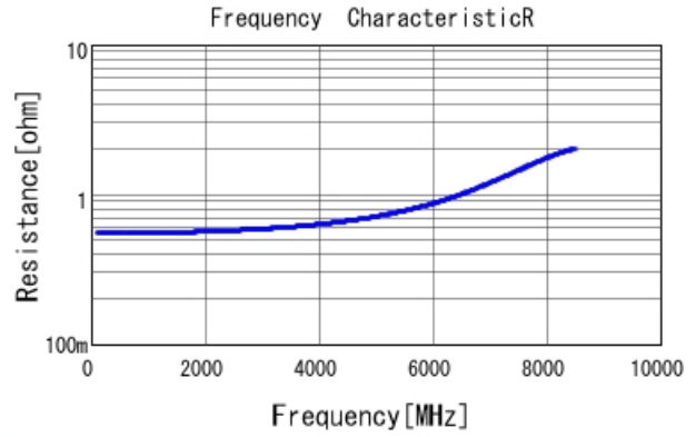
GRM1555C1H1R4CA01 R DCOV, 25degC
