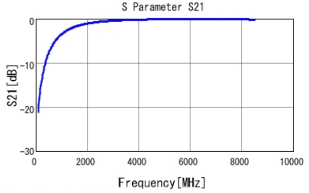
GRM1555C1H1R4CA01 S21 DCOV, 25degC
