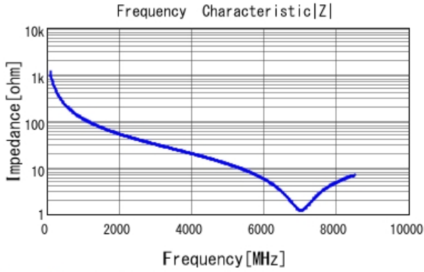
GRM1555C1H1R4CA01 |Z| DCOV, 25degC
