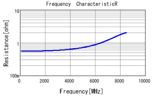
GRM1555C1H1R5WA01 R DCOV, 25degC
