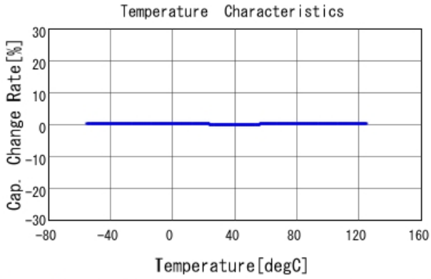
GRM1555C1H1R5WA01 C-Temp. capchange, DC0V, AC1Vrms
