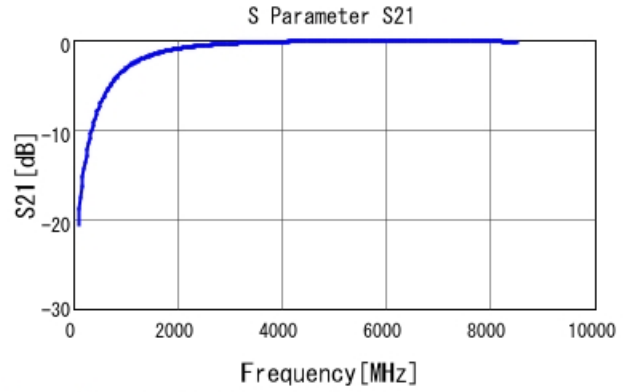
GRM1555C1H1R5WA01 S21 DC0V, 25degC
