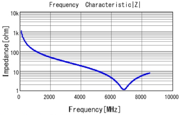
GRM1555C1H1R5WA01 |Z| DCOV, 25degC
