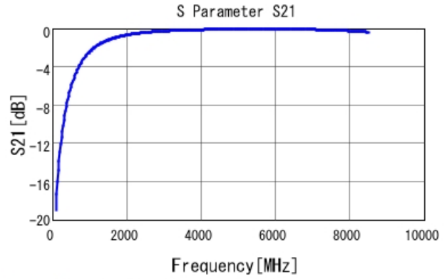
GRM1555C1H1R8WA01 S21 DCOV, 25degC
