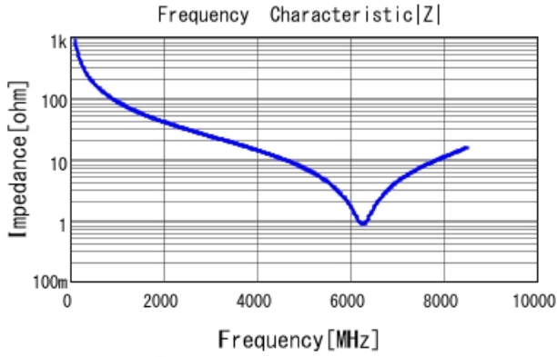
GRM1555C1H1R8WA01 |Z| DCOV, 25degC
