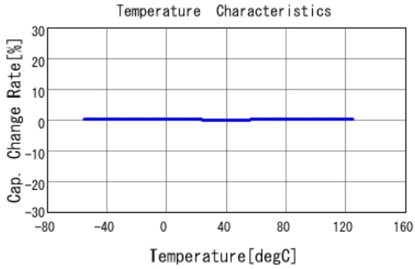
GRM1555C1H1R8WA01 C-Temp. capchange, DCOV, AC1Vrms
