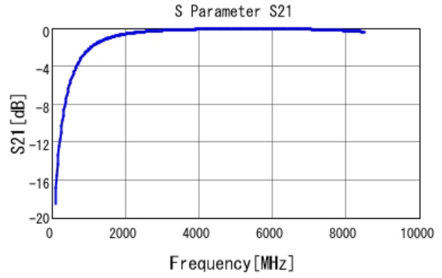
GRM1555C1H1R9WA01 S21 DCOV, 25degC
