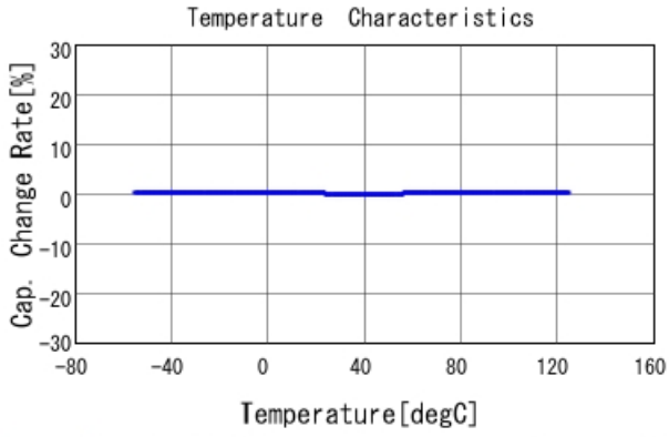
GRM1555C1H1R9WA01 C-Temp. capchange, DCOV, AC1Vrms
