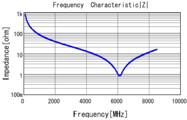
GRM1555C1H1R9WA01 |Z| DCOV, 25degC
