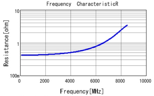
GRM1555C1H1R9WA01 R DCOV, 25degC
