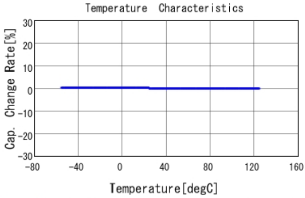
GRM1555C1H270JA01 C-Temp. capchange, DCOV, AC1Vrms
