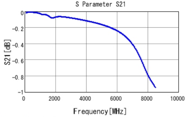
GRM1555C1H271GA01 S21 DCOV, 25degC
