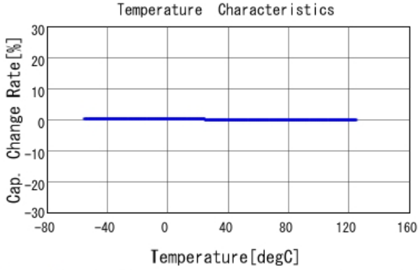
GRM1555C1H271GA01 C-Temp. capchange, DCOV, AC1Vrms
