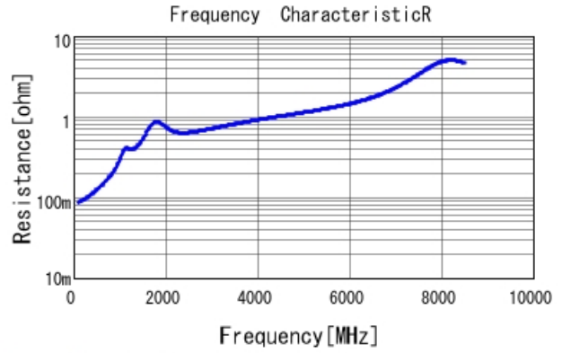
GRM1555C1H271GA01 R DCOV, 25degC
