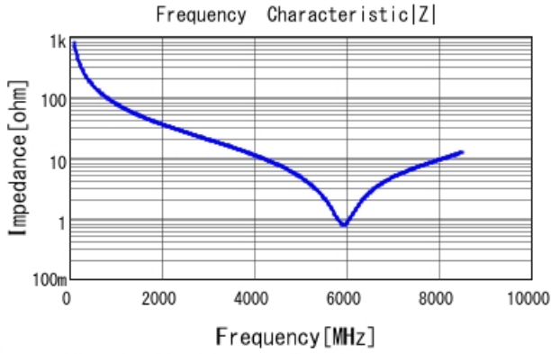
GRM1555C1H2R0CA01 |Z| DCOV, 25degC
