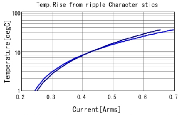
GRM1555C1H2R0CA01 Temp. rise — 2GHz — 3GHz
