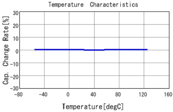
GRM1555C1H2R0CA01 C-Temp. capchange, DCOV, AC1Vrms
