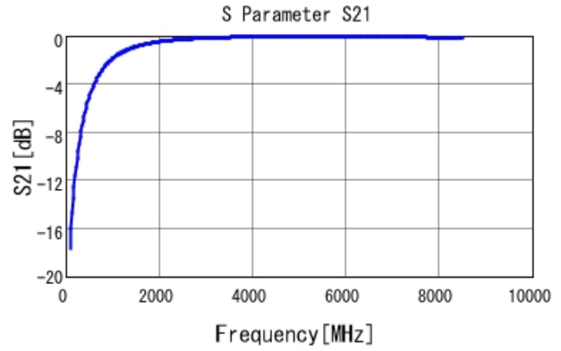
GRM1555C1H2R1WA01 S21 DCOV, 25degC
