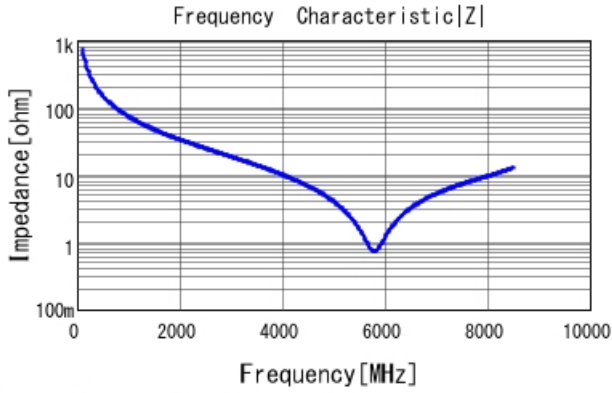
GRM1555C1H2R1WA01 |Z| DCOV, 25degC
