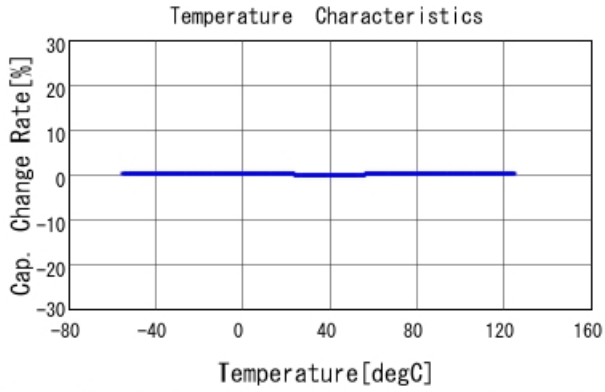
GRM1555C1H2R1WA01 C-Temp. capchange, DCOV, AC1Vrms
