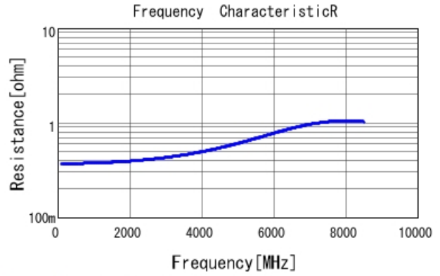
GRM1555C1H2R1WA01 R DCOV, 25degC
