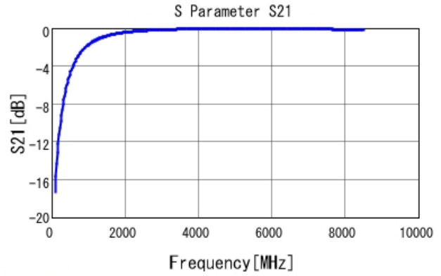
GRM1555C1H2R2WA01 S21 DCOV, 25degC
