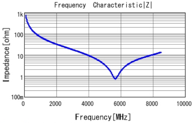
GRM1555C1H2R2WA01 |Z| DCOV, 25degC
