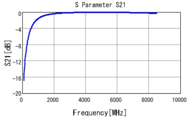
GRM1555C1H2R3BA01 S21 DCOV, 25degC
