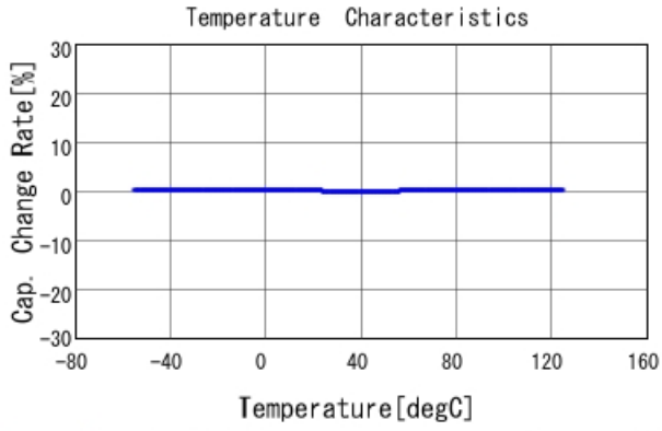
GRM1555C1H2R3BA01 C-Temp. capchange, DCOV, AC1Vrms
