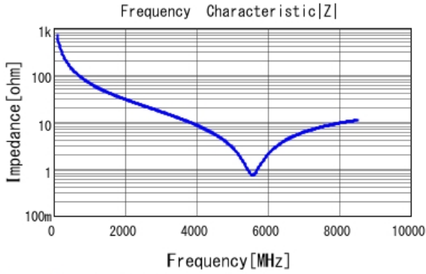
GRM1555C1H2R3BA01 |Z| DCOV, 25degC
