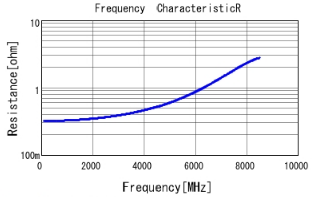
GRM1555C1H2R3BA01 R DCOV, 25degC
