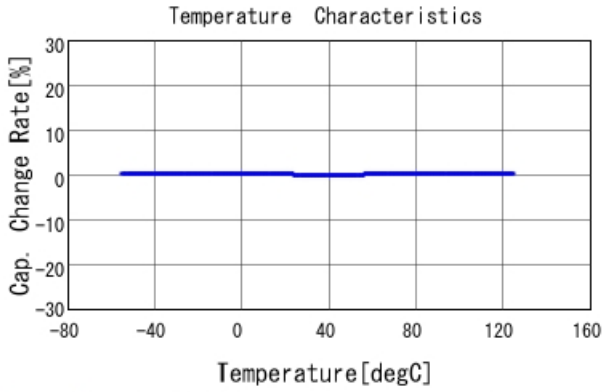
GRM1555C1H2R6CA01 C-Temp. capchange, DCOV, AC1Vrms
