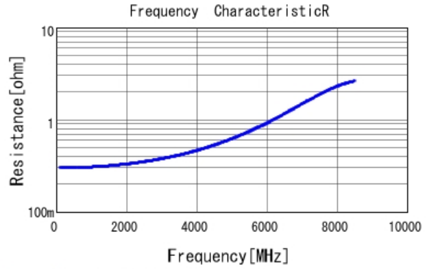
GRM1555C1H2R6CA01 R DCOV, 25degC
