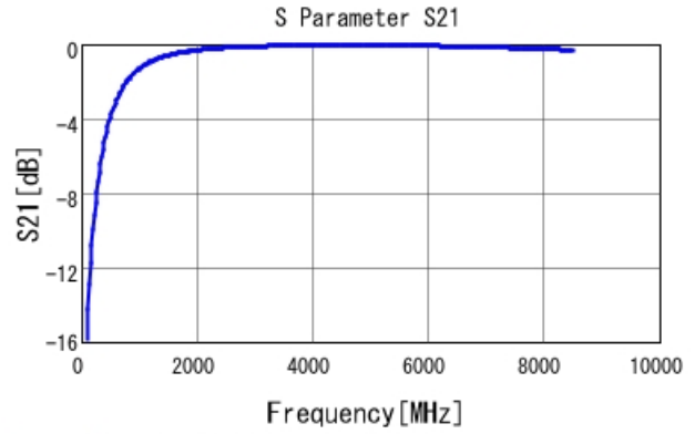
GRM1555C1H2R6CA01 S21 DCOV, 25degC
