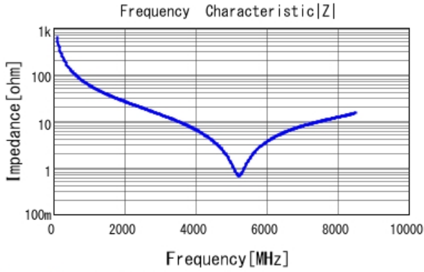
GRM1555C1H2R6CA01 |Z| DCOV, 25degC
