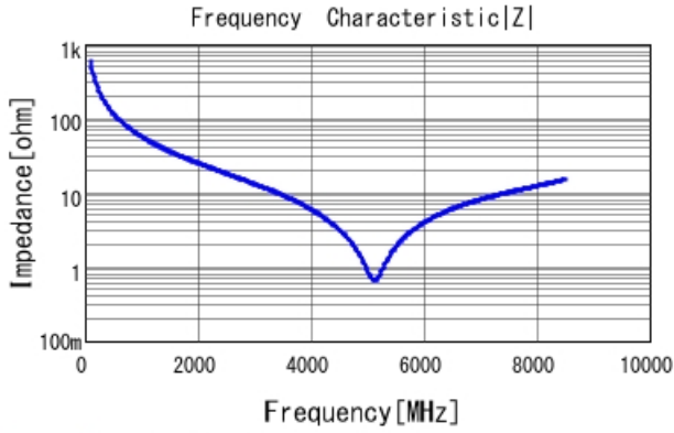
GRM1555C1H2R7BA01 |Z| DCOV, 25degC
