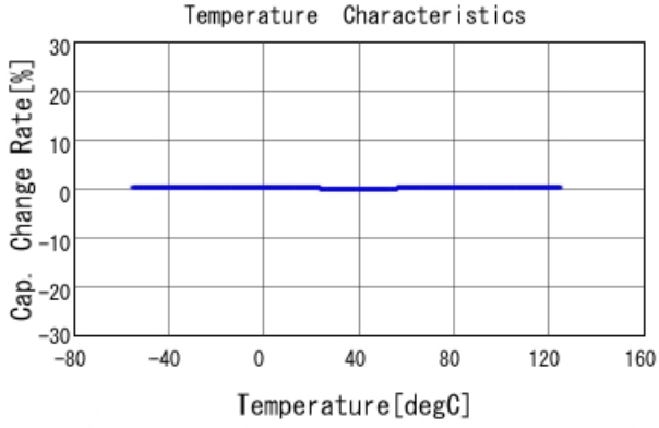
GRM1555C1H2R7BA01 C-Temp. capchange, DCOV, AC1Vrms
