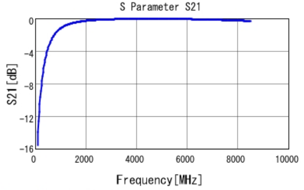
GRM1555C1H2R7BA01 S21 DCOV, 25degC
