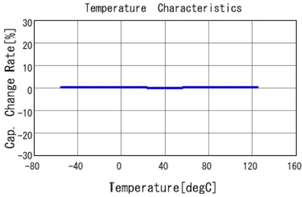
GRM1555C1H2R7CA01 C-Temp. capchange, DCOV, AC1Vrms
