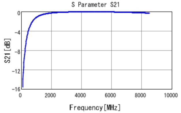
GRM1555C1H2R7CA01 S21 DCOV, 25degC
