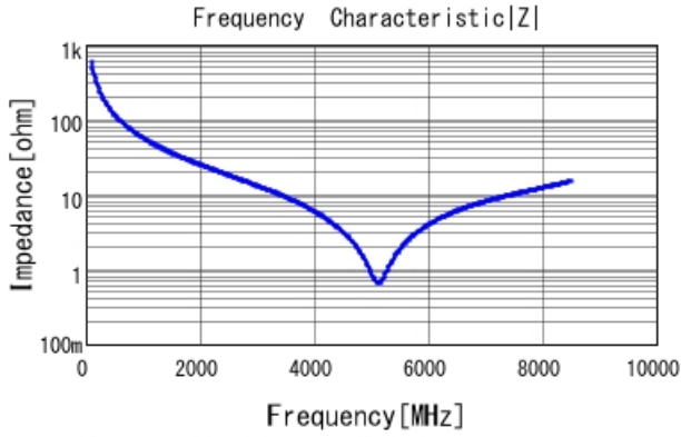
GRM1555C1H2R7CA01 |Z| DCOV, 25degC
