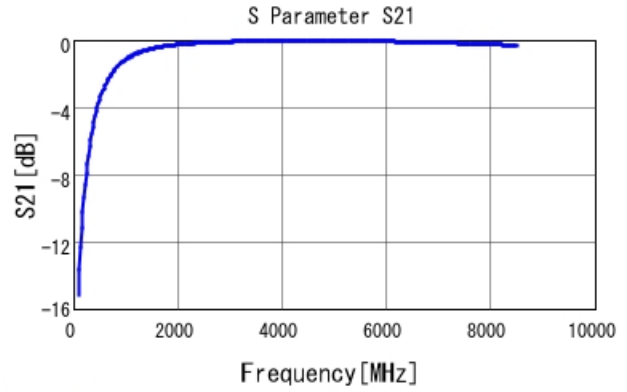
GRM1555C1H2R8CA01 S21 DCOV, 25degC
