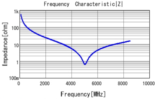
GRM1555C1H2R8CA01 |Z| DCOV, 25degC
