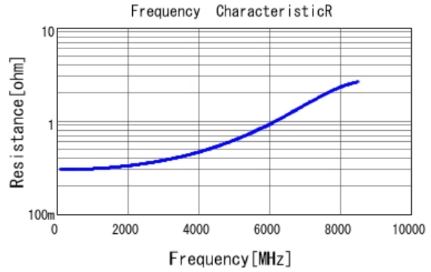
GRM1555C1H2R8CA01 R DCOV, 25degC
