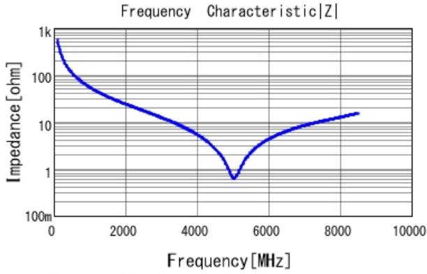
GRM1555C1H2R8WA01 |Z| DCOV, 25degC
