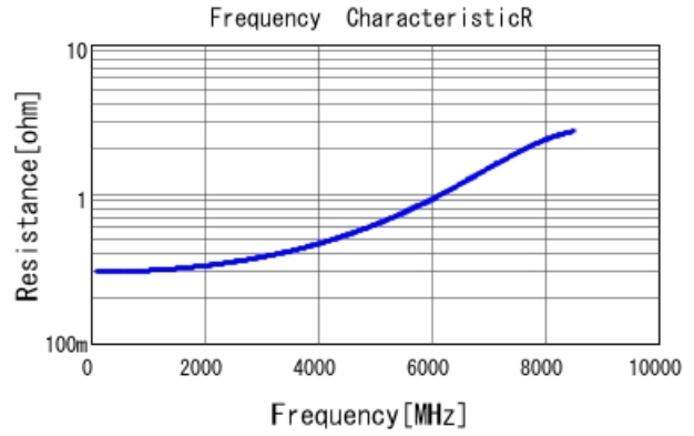
GRM1555C1H2R8WA01 R DCOV, 25degC
