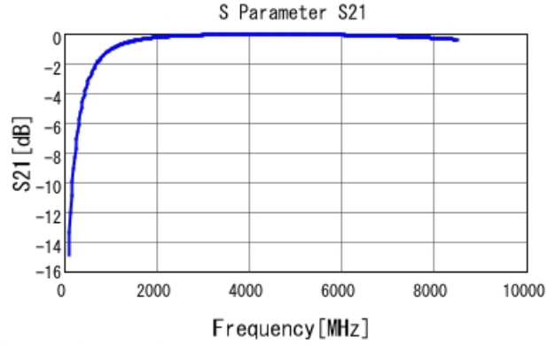
GRM1555C1H2R9WA01 S21 DCOV, 25degC
