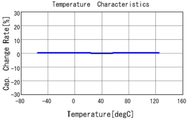
GRM1555C1H2R9WA01 C-Temp. capchange, DCOV, AC1Vrms
