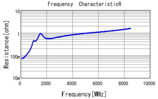
GRM1555C1H331GA01 R DCOV, 25degC
