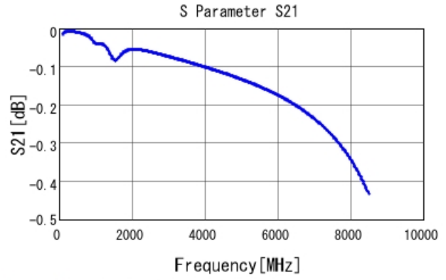
GRM1555C1H331JA01 S21 DCOV, 25degC
