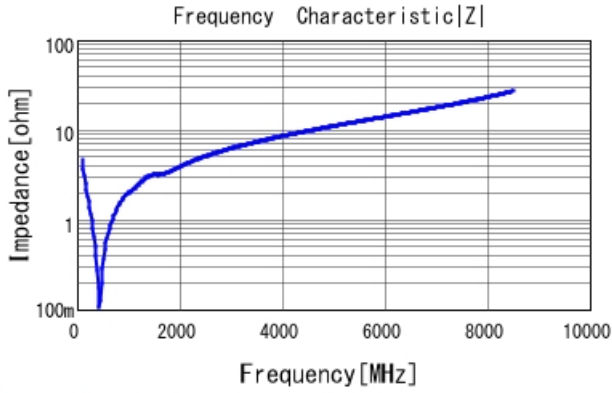
GRM1555C1H331JA01 |Z| DCOV, 25degC
