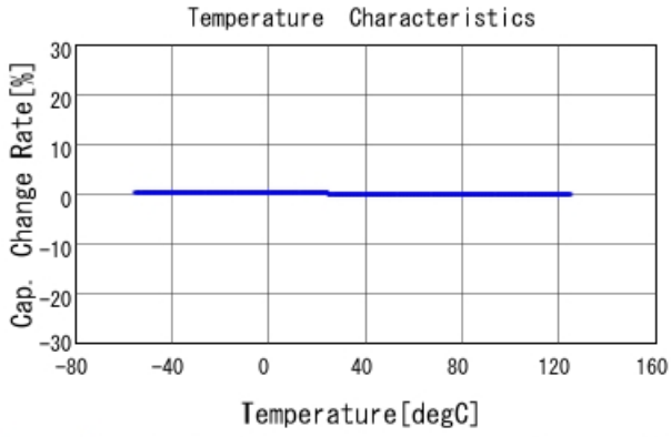
GRM1555C1H331JA01 C-Temp. capchange, DCOV, AC1Vrms
