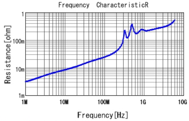
GRM1555C1H332GE01 R DCOV, 25degC
