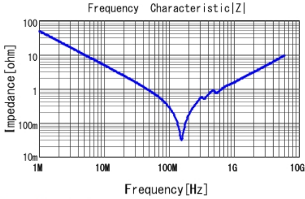
GRM1555C1H332GE01 |Z| DCOV, 25degC
