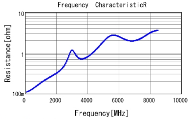
GRM1555C1H360JA01 R DCOV, 25degC
