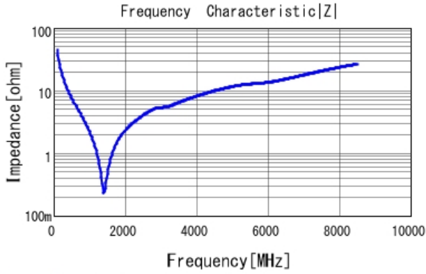
GRM1555C1H360JA01 |Z| DCOV, 25degC
