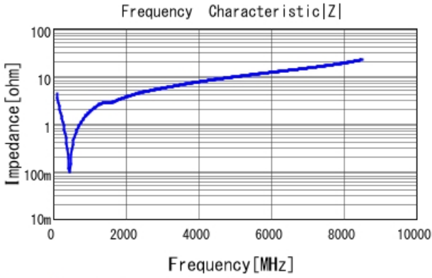
GRM1555C1H361JA01 |Z| DCOV, 25degC
