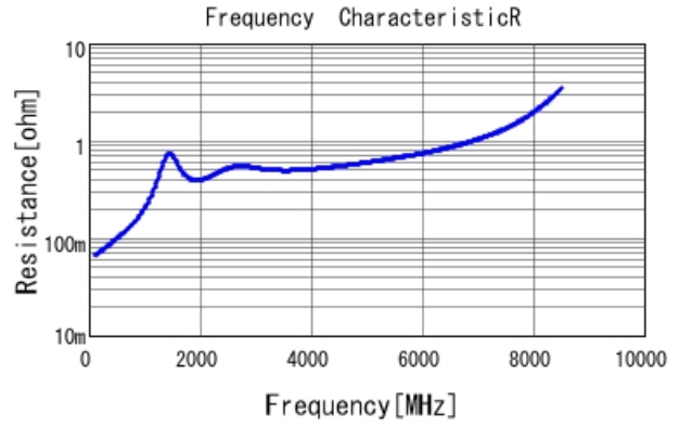
GRM1555C1H361JA01 R DCOV, 25degC
