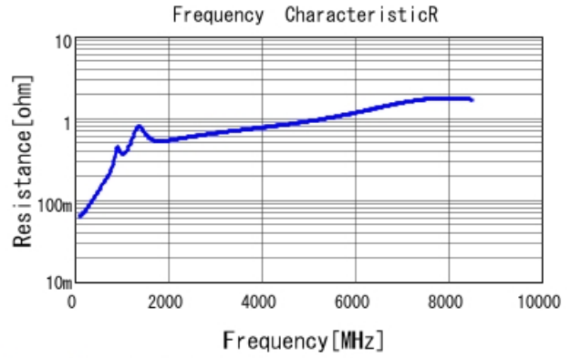
GRM1555C1H391GA01 R DCOV, 25degC
