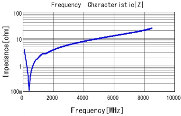
GRM1555C1H391GA01 |Z| DCOV, 25degC
