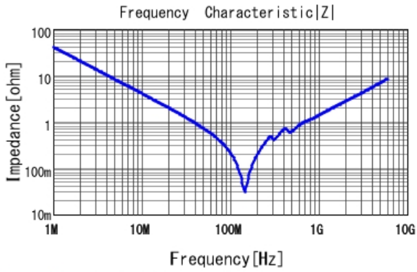
GRM1555C1H392JE01 |Z| DCOV, 25degC
