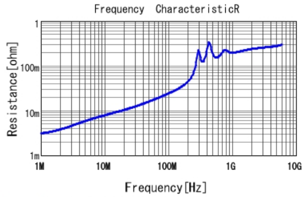
GRM1555C1H392JE01 R DCOV, 25degC
