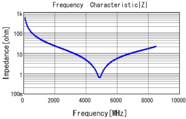
GRM1555C1H3R0BA01 |Z| DCOV, 25degC
