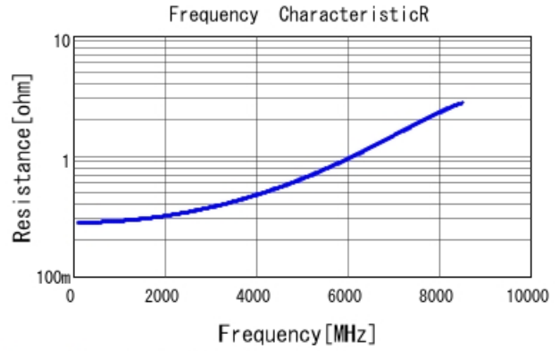
GRM1555C1H3R0BA01 R DCOV, 25degC
