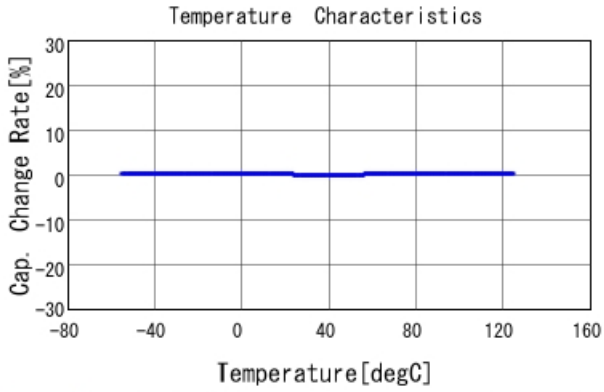
GRM1555C1H3R0BA01 C-Temp. capchange, DCOV, AC1Vrms
