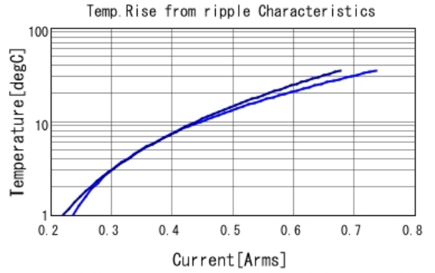
GRM1555C1H3R0BA01 Temp. rise — 2GHz — 3GHz
