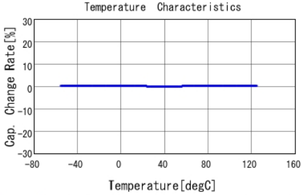
GRM1555C1H3R2WA01 C-Temp. capchange, DCOV, AC1Vrms
