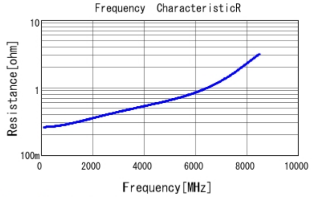
GRM1555C1H3R2WA01 R DCOV, 25degC
