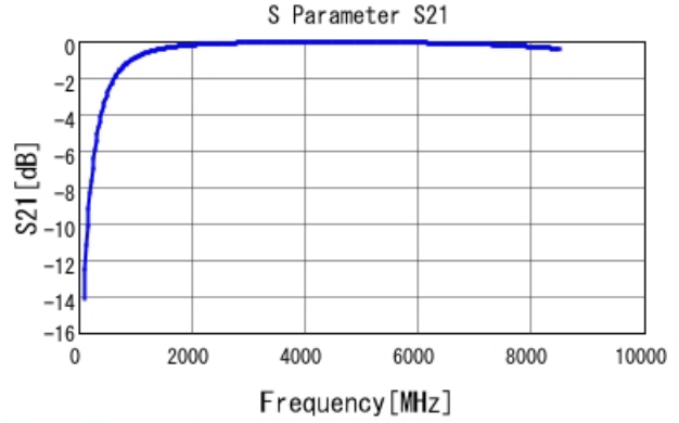
GRM1555C1H3R2WA01 S21 DCOV, 25degC
