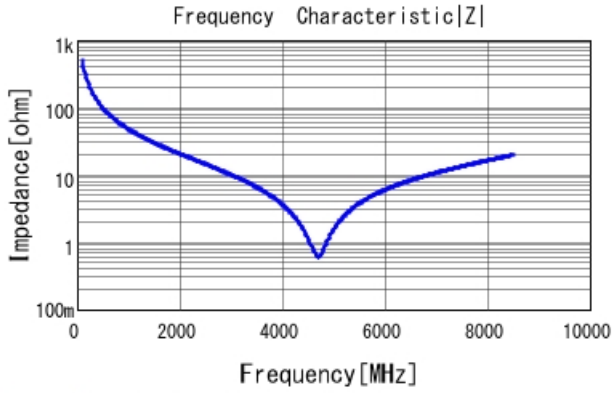
GRM1555C1H3R2WA01 |Z| DCOV, 25degC
