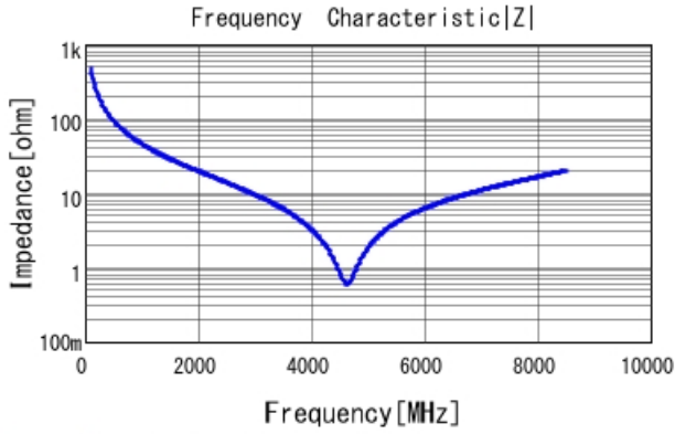
GRM1555C1H3R3CA01 |Z| DCOV, 25degC
