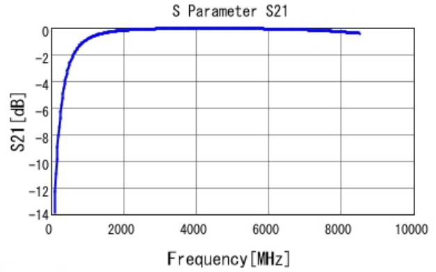
GRM1555C1H3R3CA01 S21 DCOV, 25degC
