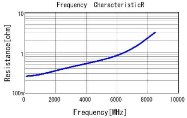
GRM1555C1H3R3CA01 R DCOV, 25degC
