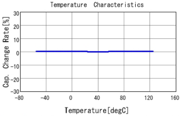
GRM1555C1H3R3CA01 C-Temp. capchange, DCOV, AC1Vrms
