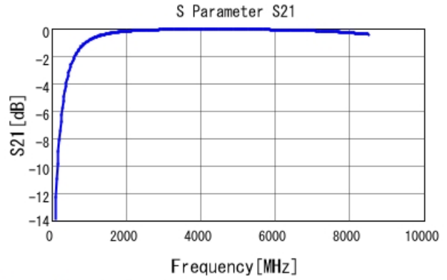
GRM1555C1H3R3WA01 S21 DCOV, 25degC
