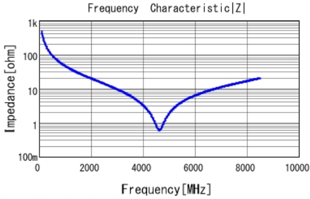
GRM1555C1H3R3WA01 |Z| DCOV, 25degC
