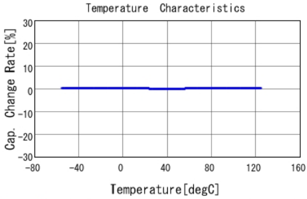
GRM1555C1H3R3WA01 C-Temp. capchange, DCOV, AC1Vrms
