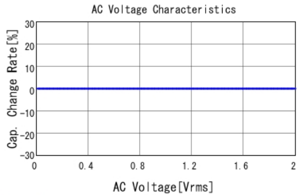
GRM1555C1H3R3WA01 C-AC Voltage capchange, DCOV, 25
