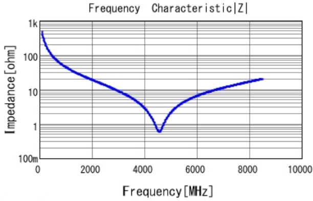
GRM1555C1H3R4CA01 |Z| DCOV, 25degC
