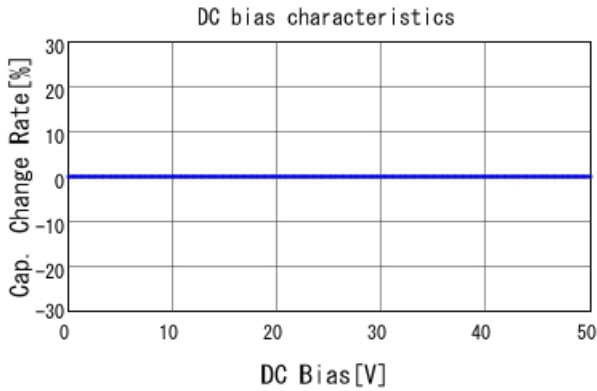
GRM1555C1H3R4CA01 C-DC bias capchange, 25.0degC, A
