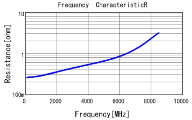
GRM1555C1H3R4WA01 R DCOV, 25degC
