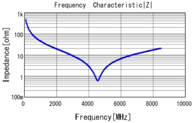
GRM1555C1H3R4WA01 |Z| DCOV, 25degC
