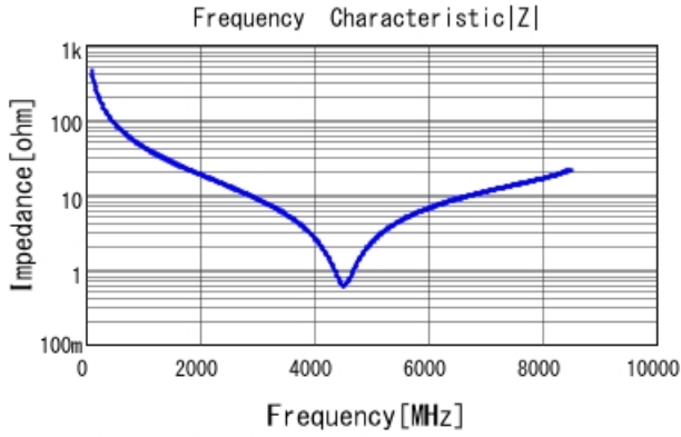
GRM1555C1H3R5WA01 |Z| DCOV, 25degC
