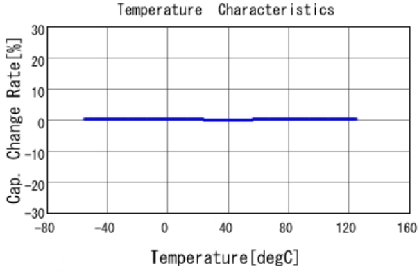
GRM1555C1H3R5WA01 C-Temp. capchange, DC0V, AC1Vrms
