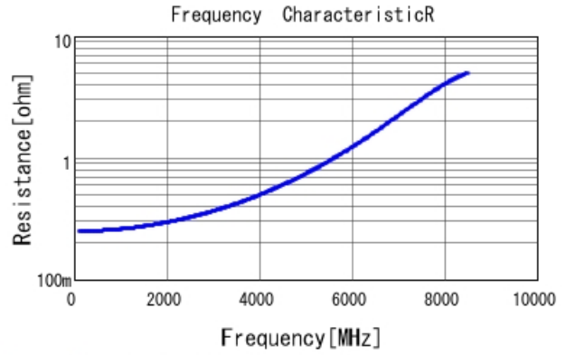
GRM1555C1H3R5WA01 R DCOV, 25degC
