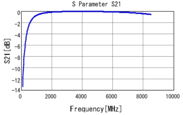
GRM1555C1H3R5WA01 S21 DC0V, 25degC
