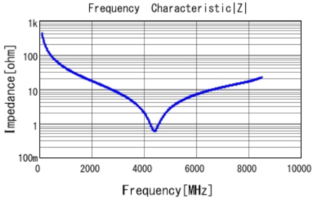
GRM1555C1H3R7CA01 |Z| DCOV, 25degC
