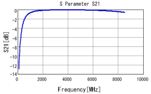
GRM1555C1H3R7CA01 S21 DCOV, 25degC
