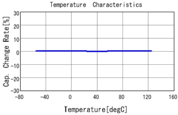
GRM1555C1H3R7CA01 C-Temp. capchange, DCOV, AC1Vrms
