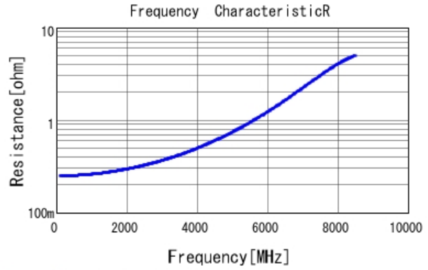
GRM1555C1H3R7CA01 R DCOV, 25degC
