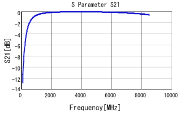
GRM1555C1H3R7WA01 S21 DCOV, 25degC
