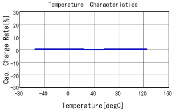
GRM1555C1H3R7WA01 C-Temp. capchange, DCOV, AC1Vrms
