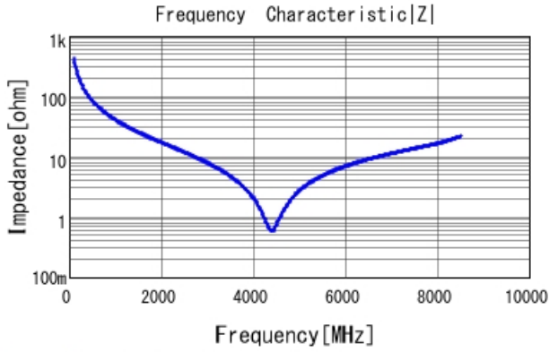
GRM1555C1H3R7WA01 |Z| DCOV, 25degC
