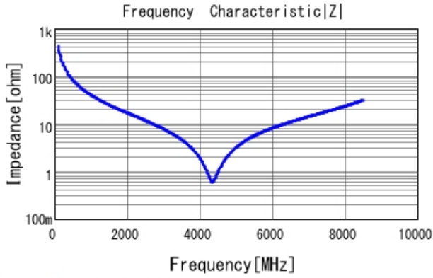
GRM1555C1H3R8BA01 |Z| DCOV, 25degC
