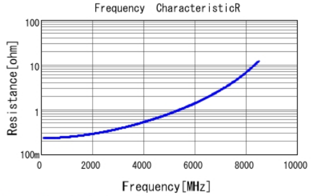
GRM1555C1H3R8BA01 R DCOV, 25degC
