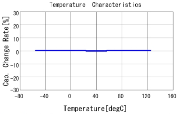
GRM1555C1H3R8BA01 C-Temp. capchange, DC0V, AC1Vrms
