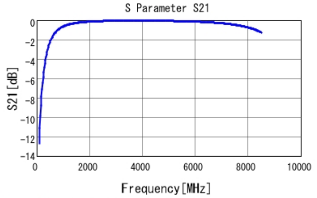
GRM1555C1H3R8BA01 S21 DC0V, 25degC
