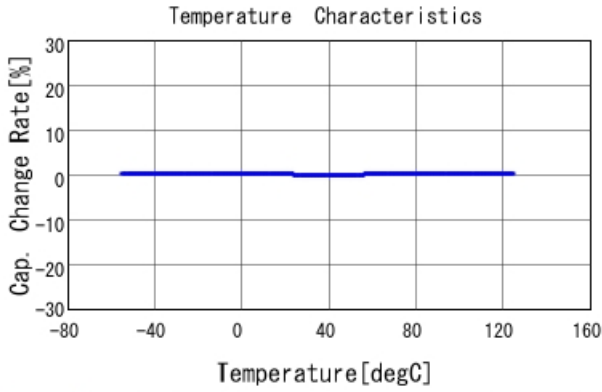
GRM1555C1H3R8CA01 C-Temp. capchange, DCOV, AC1Vrms
