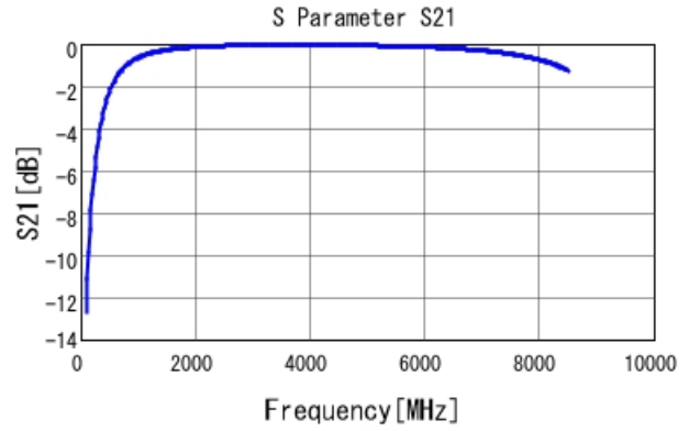
GRM1555C1H3R8CA01 S21 DCOV, 25degC
