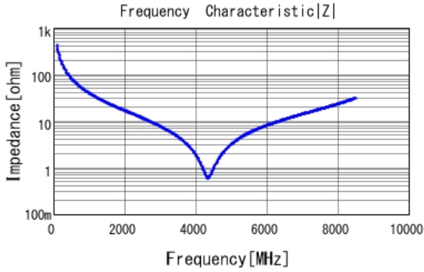
GRM1555C1H3R8WA01 |Z| DCOV, 25degC
