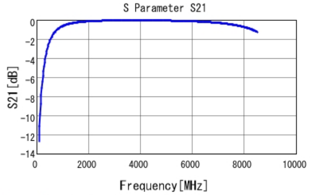
GRM1555C1H3R8WA01 S21 DCOV, 25degC
