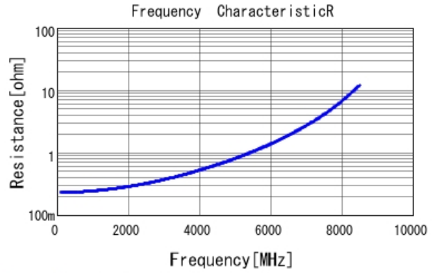
GRM1555C1H3R8WA01 R DCOV, 25degC
