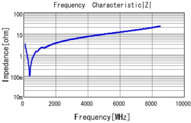
GRM1555C1H471JA01 |Z| DCOV, 25degC
