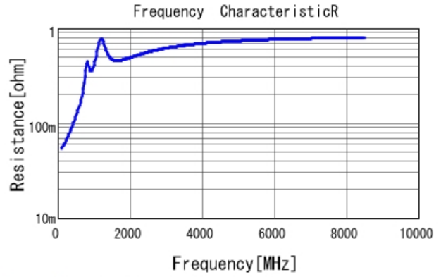
GRM1555C1H471JA01 R DCOV, 25degC
