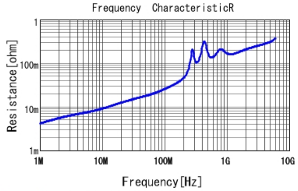
GRM1555C1H472JE01 R DCOV, 25degC
