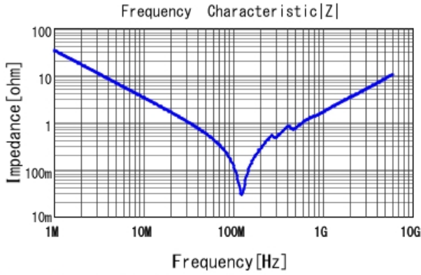
GRM1555C1H472JE01 |Z| DCOV, 25degC
