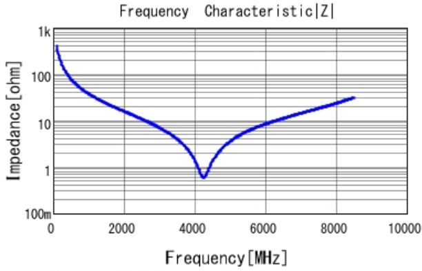
GRM1555C1H4R0BA01 |Z| DCOV, 25degC
