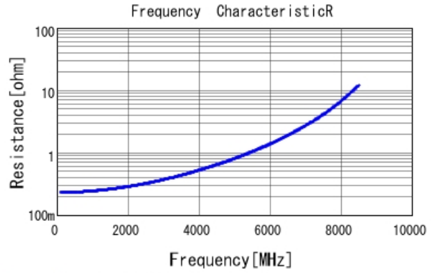
GRM1555C1H4R0BA01 R DCOV, 25degC
