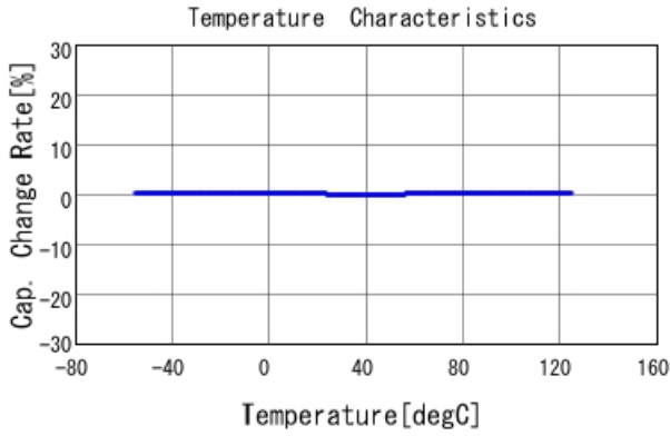
GRM1555C1H4R0BA01 C-Temp. capchange, DCOV, AC1Vrms
