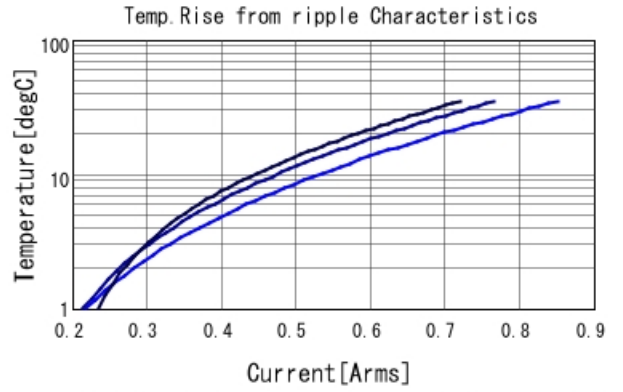
GRM1555C1H4R0BA01 Temp. rise — 1GHz — 2GHz
