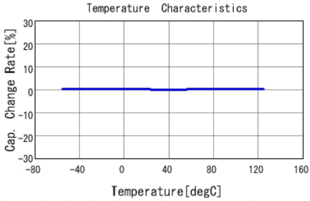
GRM1555C1H4R3BA01 C-Temp. capchange, DC0V, AC1Vrms
