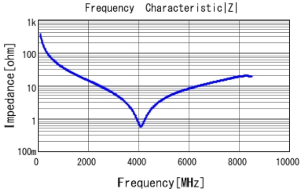
GRM1555C1H4R3BA01 |Z| DCOV, 25degC
