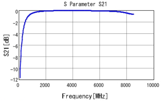
GRM1555C1H4R3BA01 S21 DC0V, 25degC
