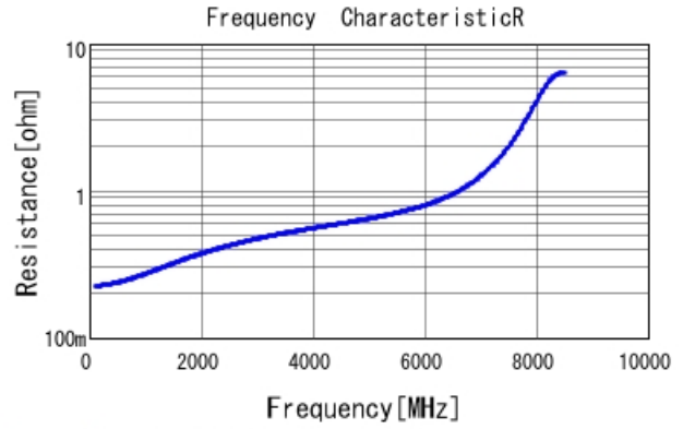
GRM1555C1H4R3BA01 R DCOV, 25degC
