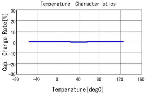
GRM1555C1H4R5CA01 C-Temp. capchange, DC0V, AC1Vrms
