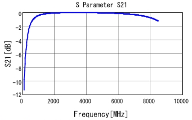
GRM1555C1H4R5CA01 S21 DC0V, 25degC
