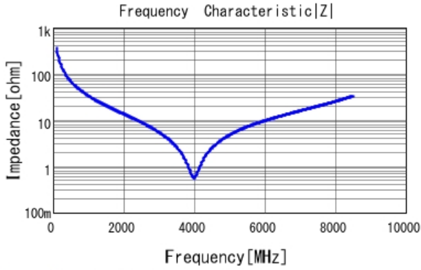
GRM1555C1H4R5CA01 |Z| DCOV, 25degC
