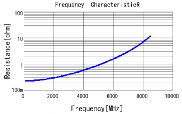
GRM1555C1H4R5CA01 R DCOV, 25degC
