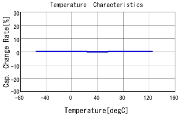
GRM1555C1H4R6BA01 C-Temp. capchange, DCOV, AC1Vrms
