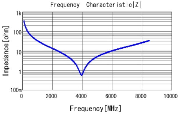
GRM1555C1H4R6BA01 |Z| DCOV, 25degC
