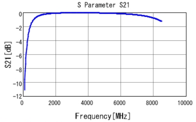
GRM1555C1H4R6BA01 S21 DCOV, 25degC
