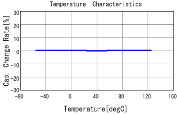
GRM1555C1H4R6CA01 C-Temp. capchange, DCOV, AC1Vrms
