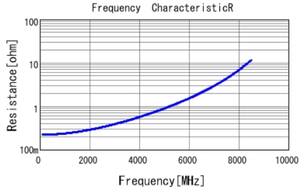
GRM1555C1H4R6CA01 R DCOV, 25degC
