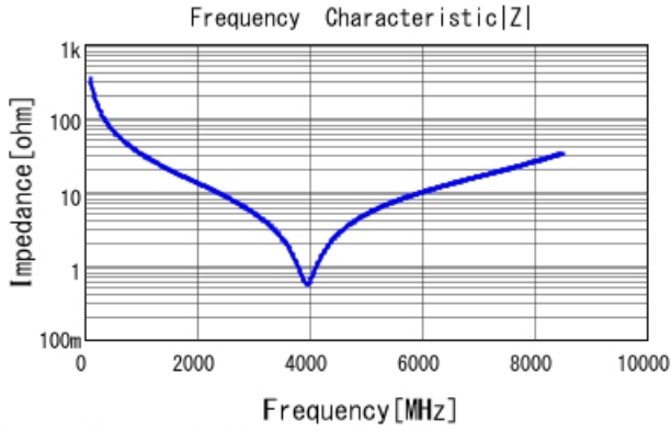
GRM1555C1H4R6CA01 |Z| DCOV, 25degC
