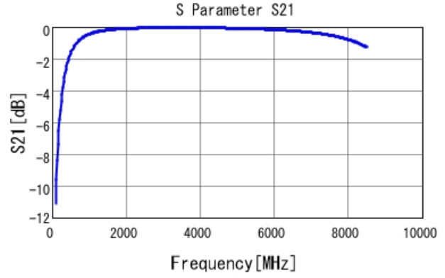
GRM1555C1H4R6CA01 S21 DCOV, 25degC
